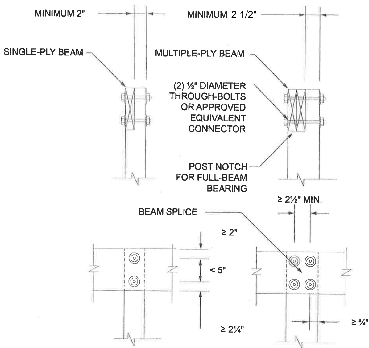
FIGURE R507.5.1(2) NOTCHED POST-TO-BEAM CONNECTION
