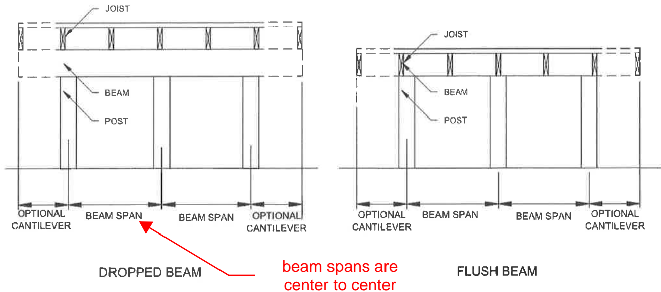
FIGURE R507.5 TYPICAL DECK JOIST SPANS
